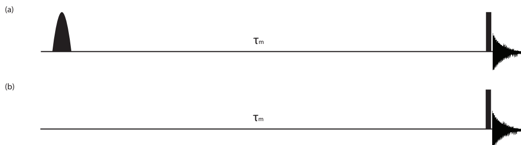
Figure 4.2: The NOE pulse sequences used in this work (a) a selective \pi sinc pulse tuned to the frequency of the isotopically enriched ^{13}\text{C} carbonyl followed by a mixing time \tau_m , a \frac{\pi}{2} broadband pulse and acquisition, and (b) a mixing time \tau_m , followed by a \frac{\pi}{2} broadband pulse and acquisition. Adapted from 9 .
