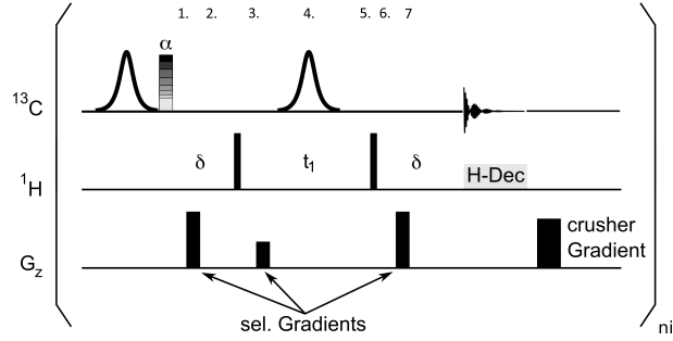
Figure 3.5: The fast 2D-HMQC pulse sequence where adiabatic \pi pulses were used on the carbon channel to avoid losses arising from B_1 inhomogeneity. The first ^{13}\text{C} flip angle, \alpha , was increased (from 10^\circ to 30^\circ ) in successive experiments to compensate for the decrease of available magnetisation for higher increments due to relaxation. Adapted from 8 .
