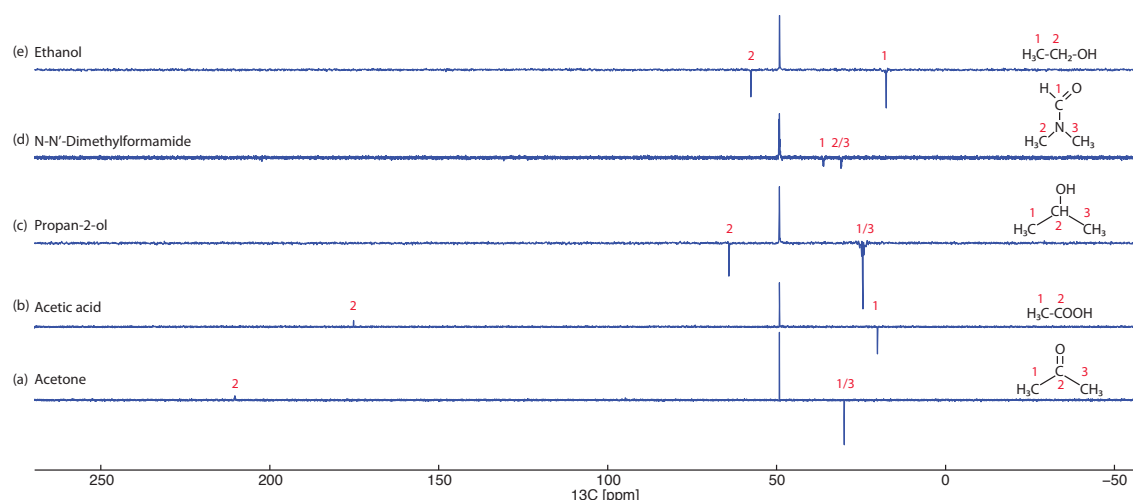
Figure 6.1: ^{13}\text{C} NMR spectrum for 100 \mu\text{l} (a) acetone, (b) acetic acid, (c) propan-2-ol, (d) N,N'-dimethyl formamide & (e) ethanol after cooling to 1.5K for 60minutes before dissolution with hot, pressurised methanol and transfer to a high field NMR spectrometer for acquisition of the NMR spectrum with a simple \pi/2 pulse followed by acquisition of the NMR spectrum.
