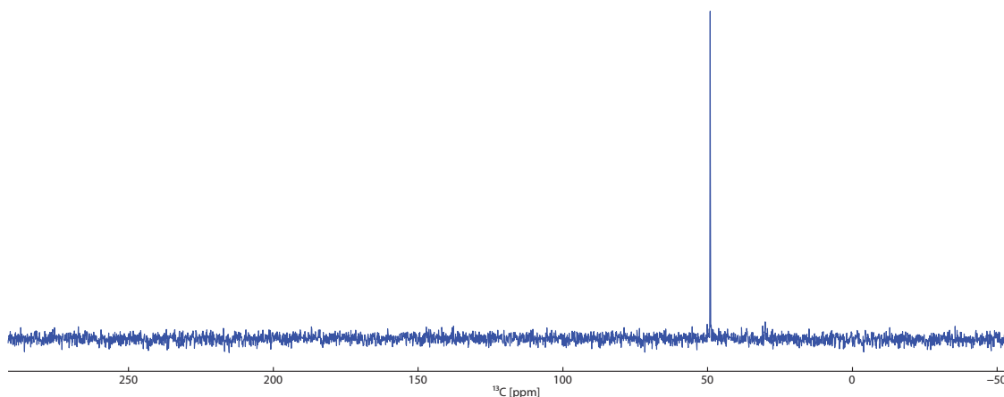
Figure 6.6: ^{13}\text{C} spectrum of an acetone pre-cooled in liquid nitrogen for 18 hours before cooling to 1.5K for 60 minutes.
