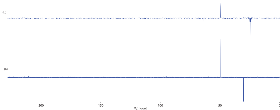
Figure 6.8: Spectra for (a) 100 \mu l acetone (b) 100 \mu l isopropanol, after cooling to 1.5K for 60minutes before dissolution with hot, pressurised methanol and transfer to a high field NMR spectrometer for acquisition of the NMR spectrum with a simple \pi/2 pulse followed by acquisition of the NMR spectrum. Enhancement values are as per table 6.1.
